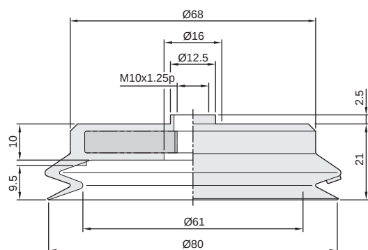
● PB-80
