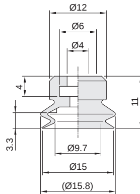
● PB-40
