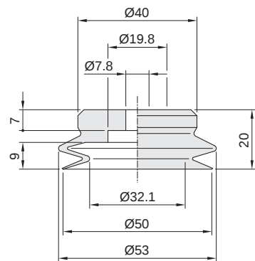
● PB-50
