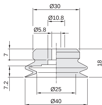
● PB-40
