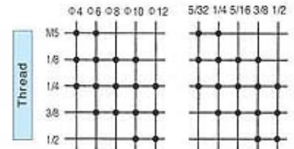
SQU Branch Y
